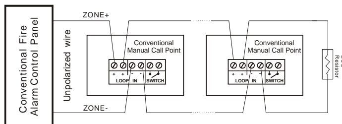
Figure 1. Install and Wiring diagram:
